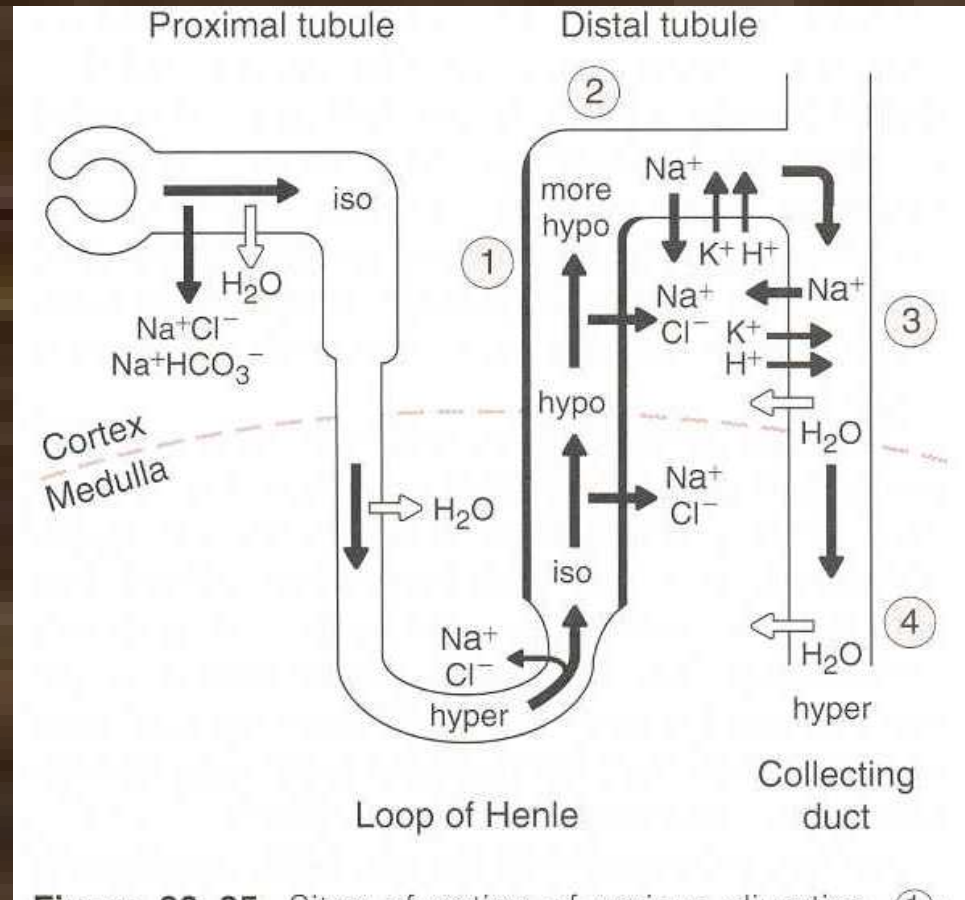
Figure 38–25. Sites of action of various diuretics. ①: Furosemide and other loop diuretics act on the thick ascending limb of the loop of Henle. ②: Thiazides act on the early portion of the distal convoluted tubule. ③: Aldosterone antagonists, triamterene, and amiloride act primarily on the collecting ducts. ④: Antagonists to V_2 vasopressin receptors act on the collecting ducts.
