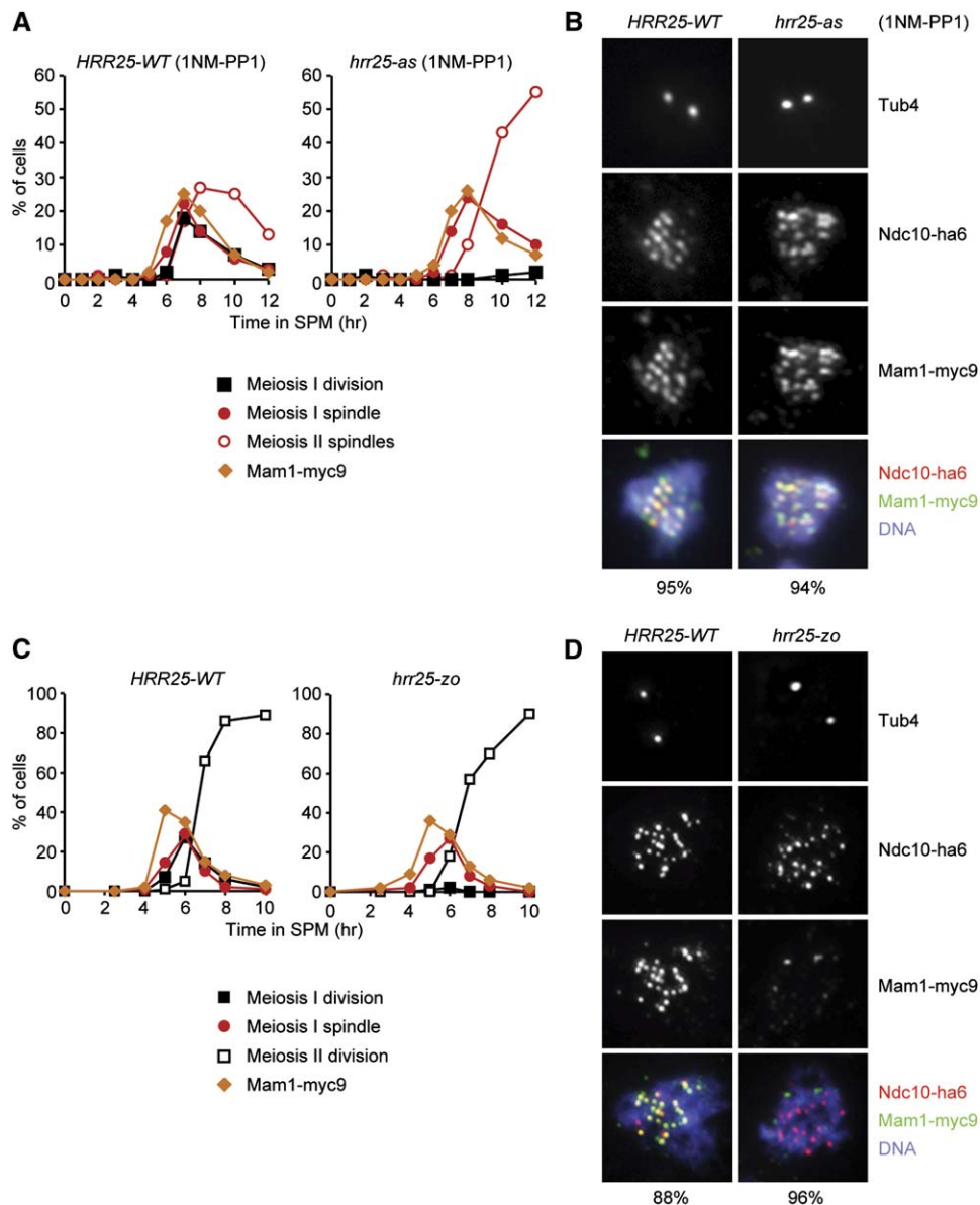
Figure 7. Mam1 Localization to Kinetochores Requires Interaction with Hrr25 but Not Hrr25's Kinase Activity
