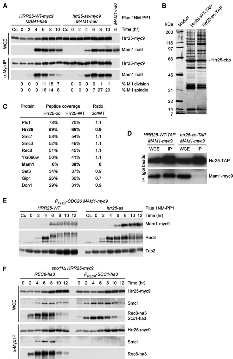
Figure 5. Interactions of Hrr25 with Mam1 and Cohesin
